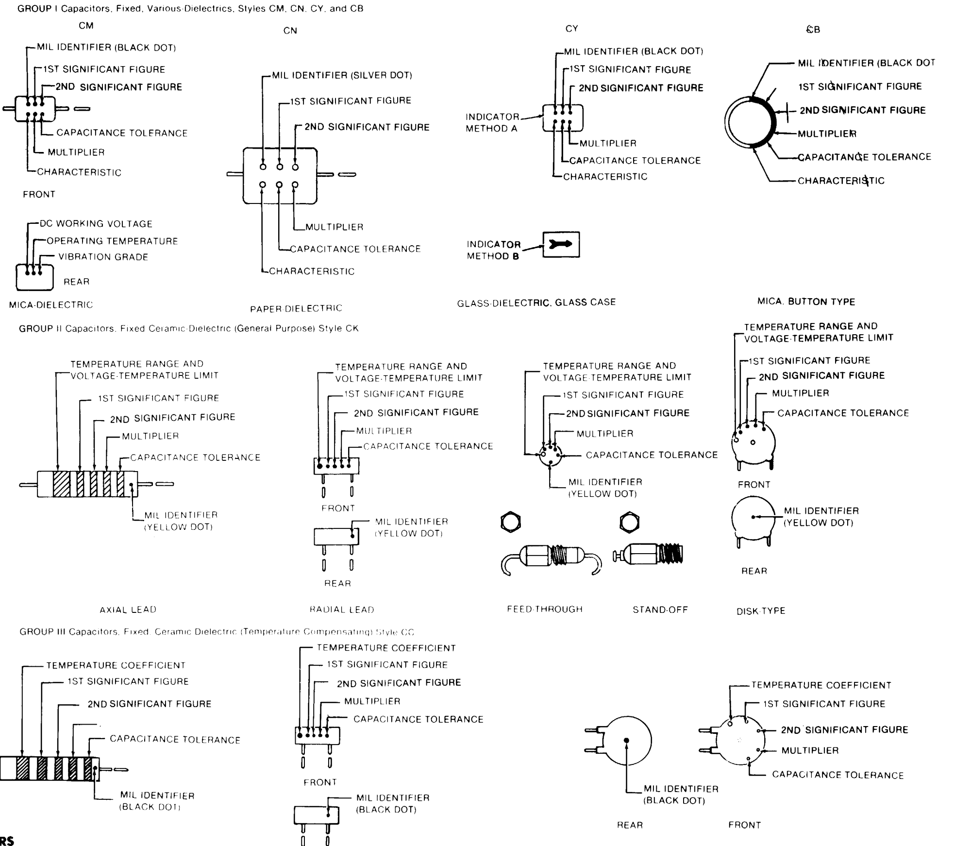
COLOR CODE MARKING FOR MILITARY STANDARD CAPACITORS
